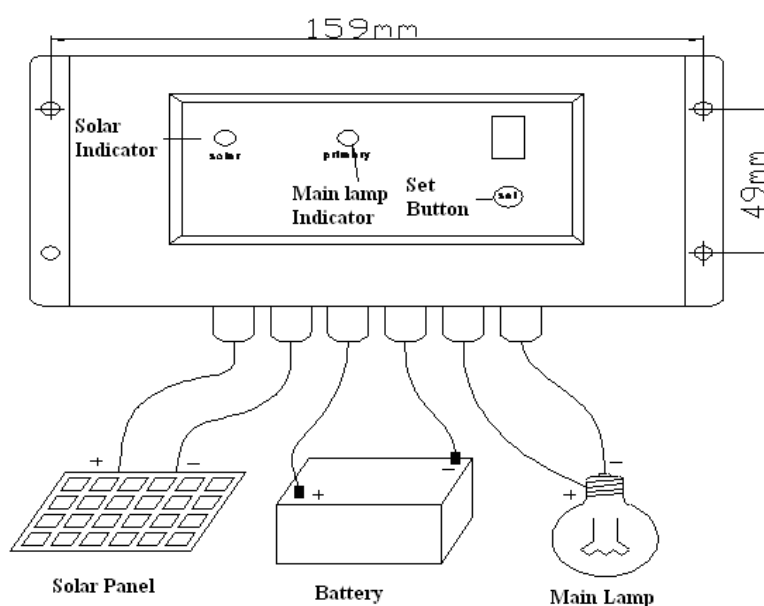
Figure-1 connection diagram of controller
